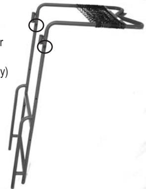
FIGURE 2 INSTALL SEATING PLATFORM ONTO UPPER LADDER 5 O'LMAN 03-2009A
