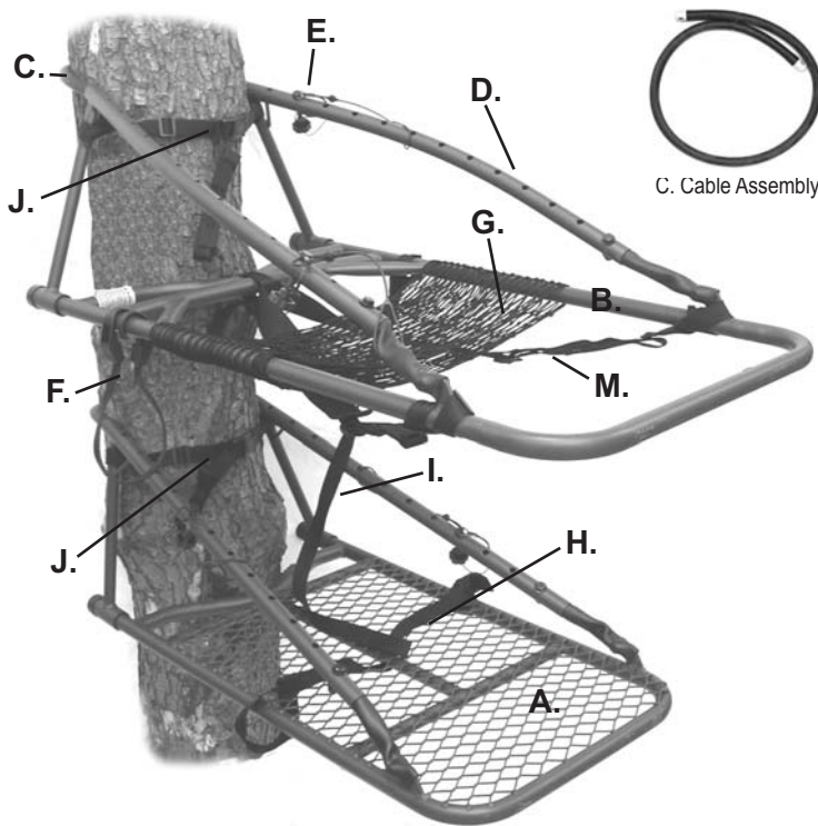
FIGURE 1 COMPONENTS OF OL' MAN TREESTANDS ORIGINAL
