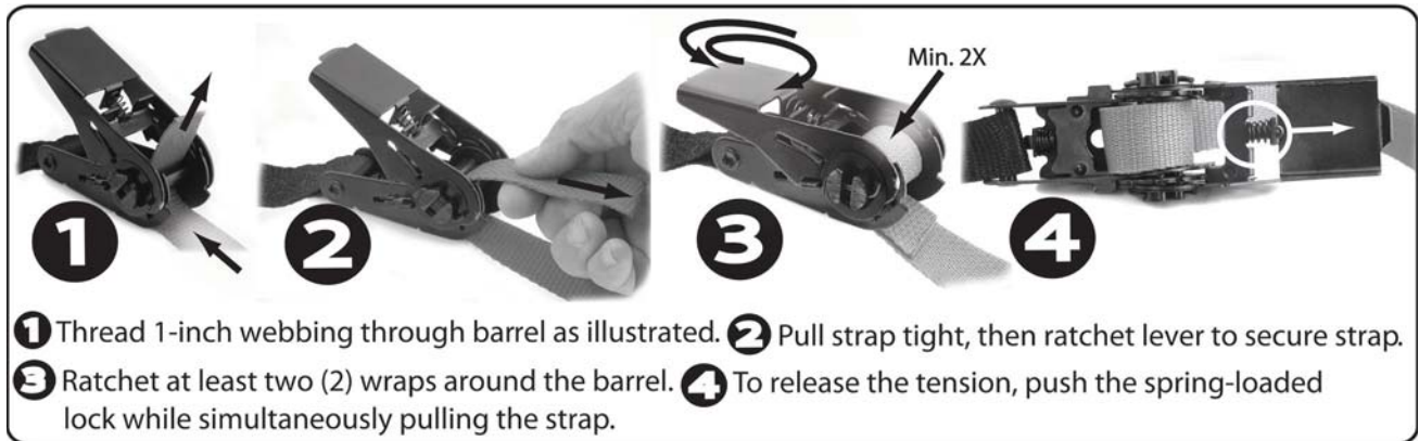
FIGURE 11 THREADING RATCHET STRAP
