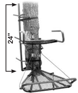
FIGURE 6 CLIMBING Aid A MINIMUM OF 24" ABOVE STANDING
